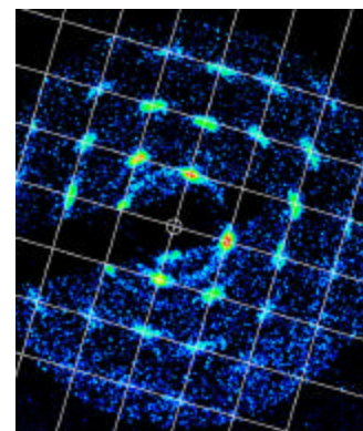
Bragg diffraction pattern of crystallized ions [W.M. Itano et al. , Science Magazine]
